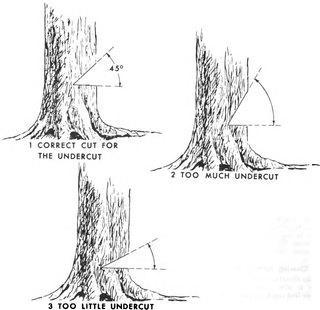
Figure 5-3. The undercut.
